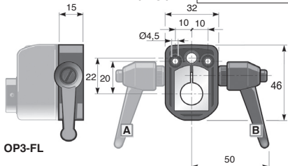
OP-FL Clamping plate
