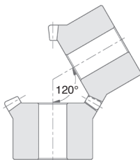
Shaft angle 120°
